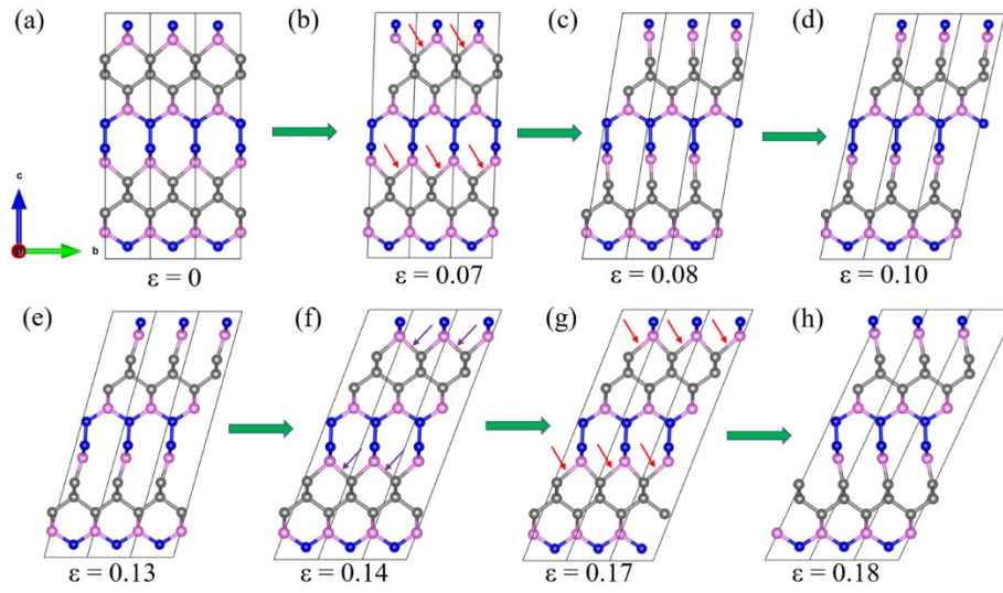
Figure S1. Structural snapshots of t\text{-B}_2\text{C}_3\text{N}_2 under the \langle 011 \rangle tensile deformation.
