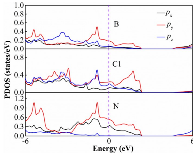
Figure S2. PDOS of p_x , p_y , and p_z orbitals for B, C1, and N atoms.
