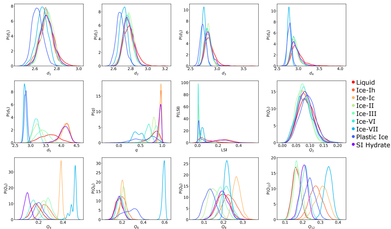
Figure S1: Distribution of order parameters composing feature vector.
