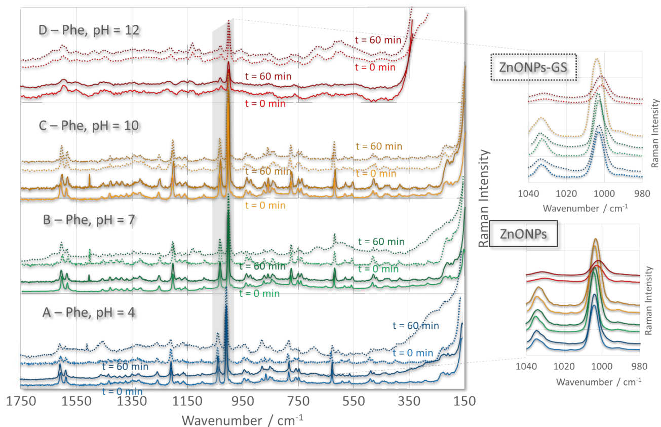
Figure 2S. SERS spectra of Phe adsorbent on ZnONPs and ZnONPs-GS at different pH and time.
