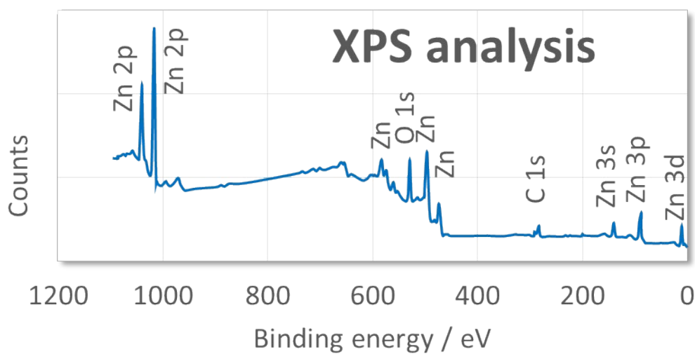
Figure 1S. XPS spectrum of ZnONPs-GC obtained from banana peels.
