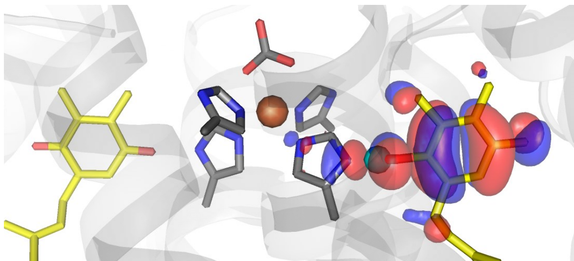
Figure S1. HOMO population of the D1-His215...Q B moiety (Q B : D1-His215 = 94.5 : 4.3) when N_{\text{His215}\dots\text{H}} = 1.44 \text{ \AA} . The HOMO is populated over Q B and D1-His215 with the ratio of 94.5 and 4.3.
