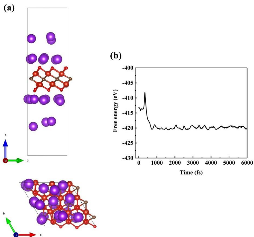
Figure S1. (a) Top and side view of snapshot after equilibration and (b) free energy as a function of MD time at the temperature of 300 K for V_2CO_2K_{2.67} .
