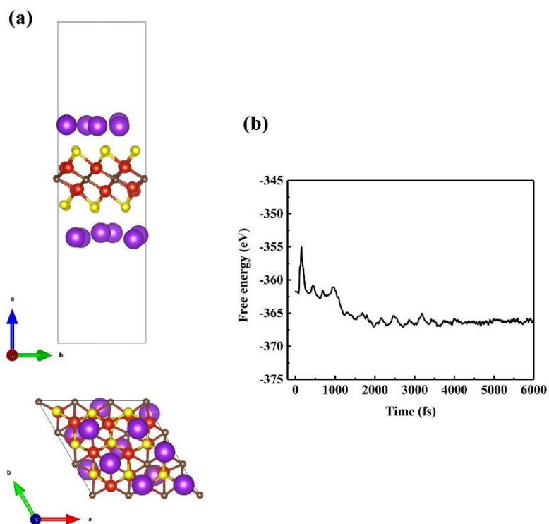
Figure S2. (a) Top and side view of snapshot after equilibration and (b) free energy as a function of MD time at the temperature of 300 K for V_2CS_2K_{1.33} .
