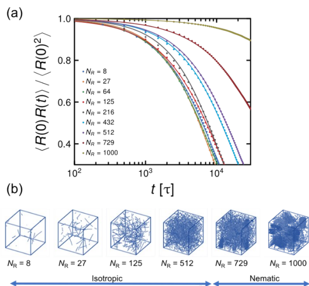
Figure A3. End-to-end vector autocorrelation function, \frac{\langle \vec{R}(0) \cdot \vec{R}(t) \rangle}{\langle R^2(0) \rangle} (a) and snapshots of simulations at different rod
