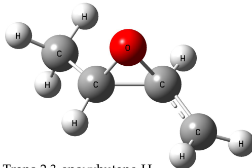
Trans-2,3-epoxybutane-H 2
