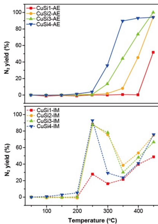
Fig. S1 N 2 yield of CuSi-AE and CuSi-IM samples as a function of the reaction temperature.
