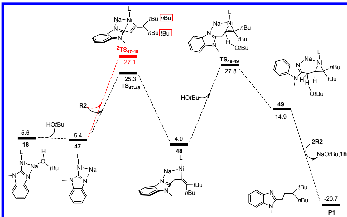
Fig. S6 Calculated free energy profile in toluene along the possible pathways starting from intermediate 18 in Fig. 2. The relative free energies are given in kcal mol -1 . L = IPr
