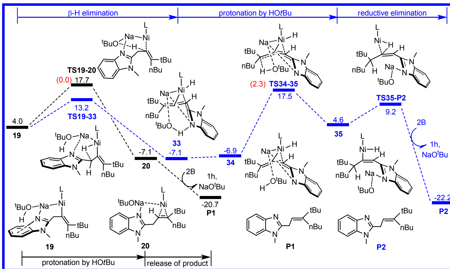
Fig. S2 Calculated free energy profiles in toluene along the possible pathways starting from intermediate 19 in Fig. 2. The optimized relative free energies in toluene solution are provided in the parentheses. The relative free energies are given in kcal mol -1 . L = IPr
