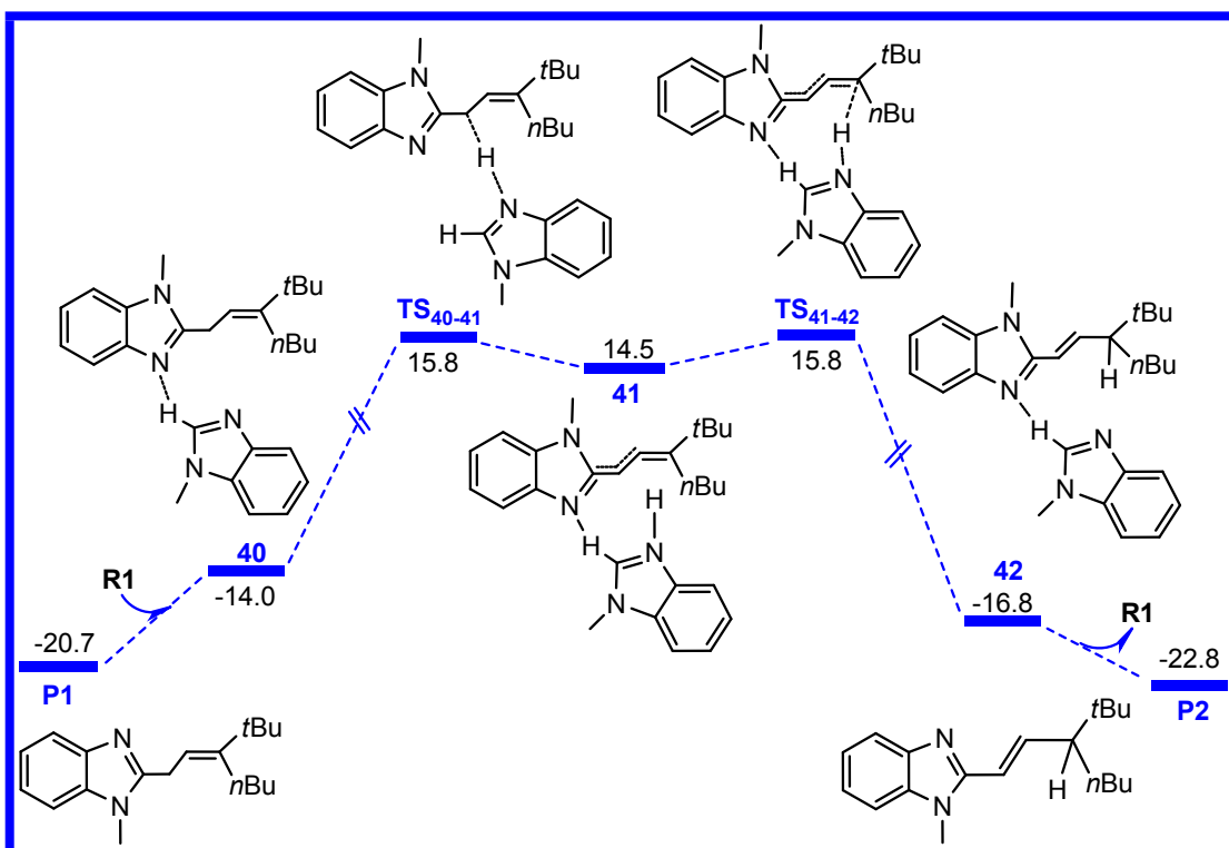
Fig. S4 Calculated free energy profile in toluene for forming P2 from P1 assisted by R1 . The relative free energies are given in kcal mol -1 .
