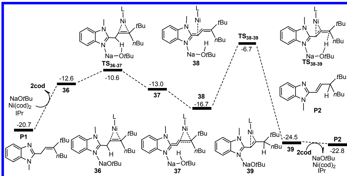
Fig. S3 Calculated free energy profile in toluene along the possible pathway for forming P2 from P1 with Ni(cod) 2 involvement in the presence of NaOtBu. The relative free energies are given in kcal mol -1 . L = IPr
