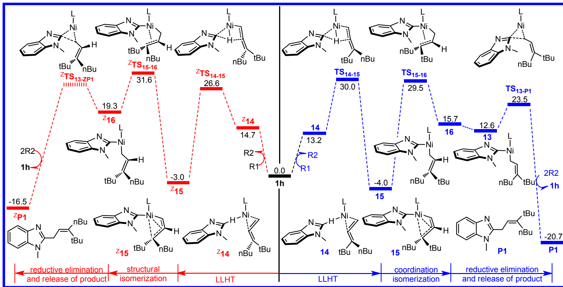
Fig. S1 Calculated free energy profiles in toluene along possible LLHT pathways in the absence of base. The relative free energies and bond distances are given in kcal mol -1 and Å, respectively.
