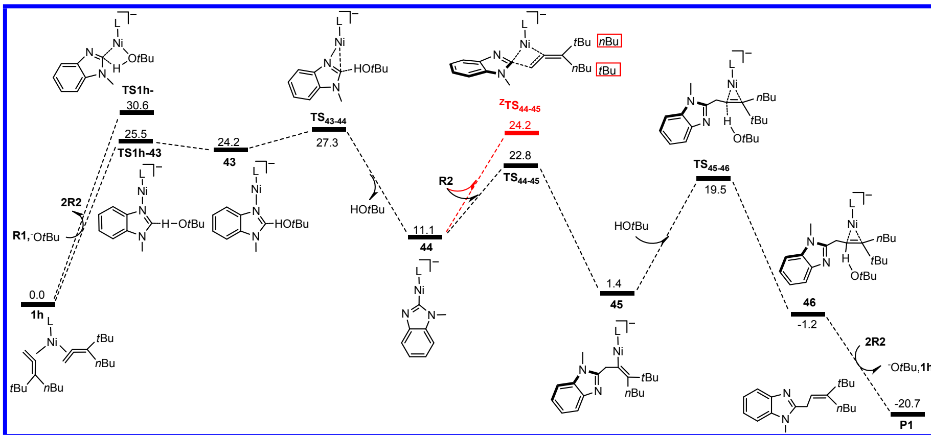
Fig. S5 Calculated free energy profiles in toluene along the possible pathways for forming P1 assisted by the \text{O}t\text{Bu} . The relative free energies are given in kcal/mol. L = IPr
