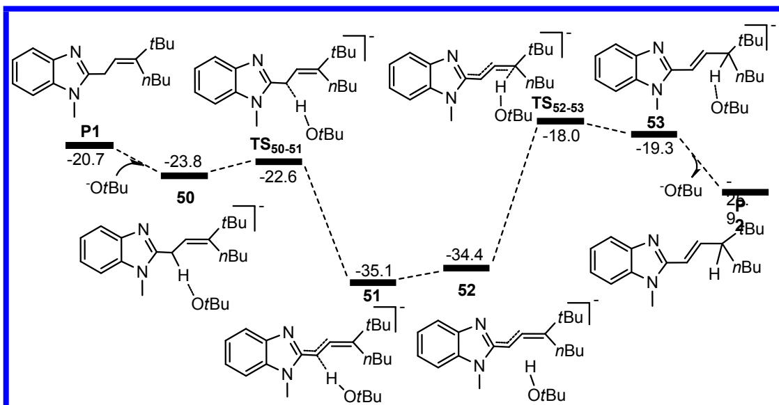
Fig. S7 Calculated free energy profile in toluene for forming P2 from P1 assisted by the - OtBu. The relative free energies are given in kcal mol -1 .
