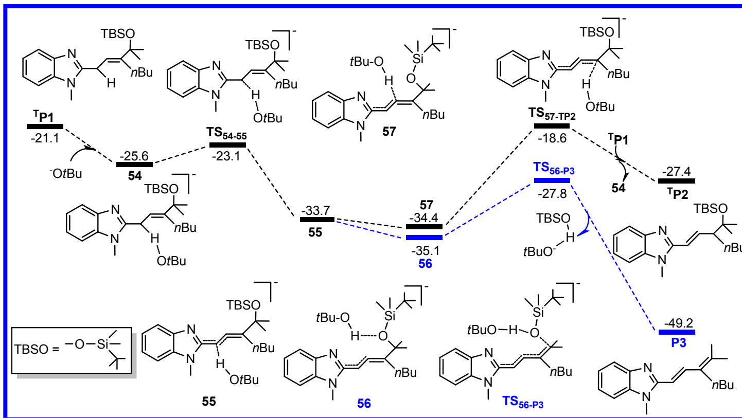
Fig. S8 Calculated free energy profiles in toluene along the possible pathways for forming TP2 and P3 , respectively, from TP1 assisted by the - O t Bu. The relative free energies are given in kcal mol -1 .
