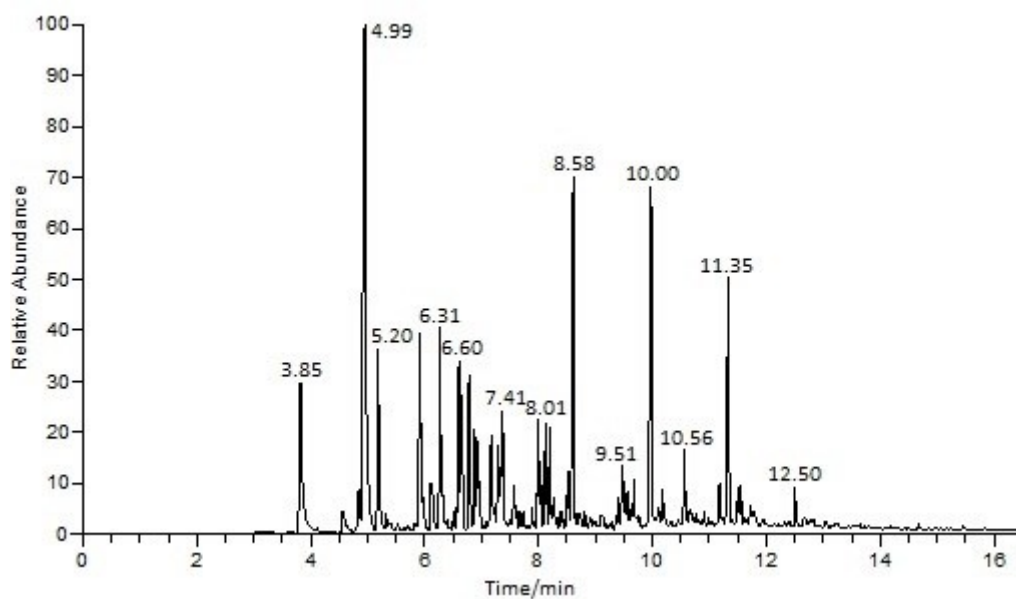
Fig.S1 The TIC spectrum of organic phase by using fresh catalyst
