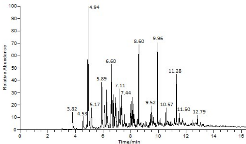
Fig.S2 The TIC spectrum of organic phase by using regenerated catalyst
