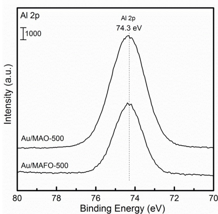
Figure S1. XPS spectra of Al 2p
