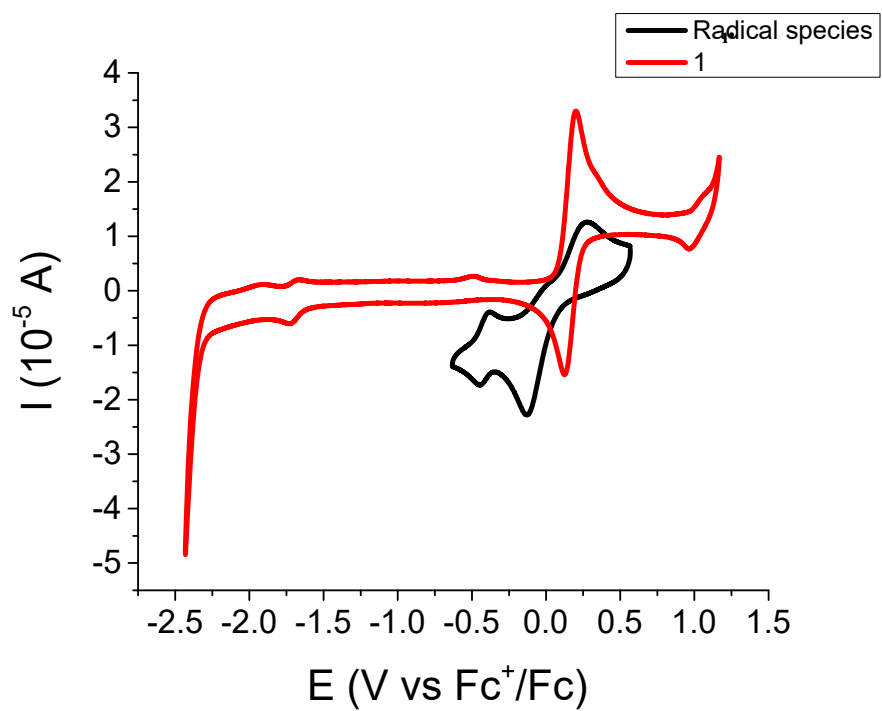
Figure S2. CVs in 2mM solution of 1 and 1 • at 0.05 V s -1 .
