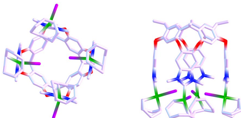
Vase_2 (1.3 kcal/mol)
