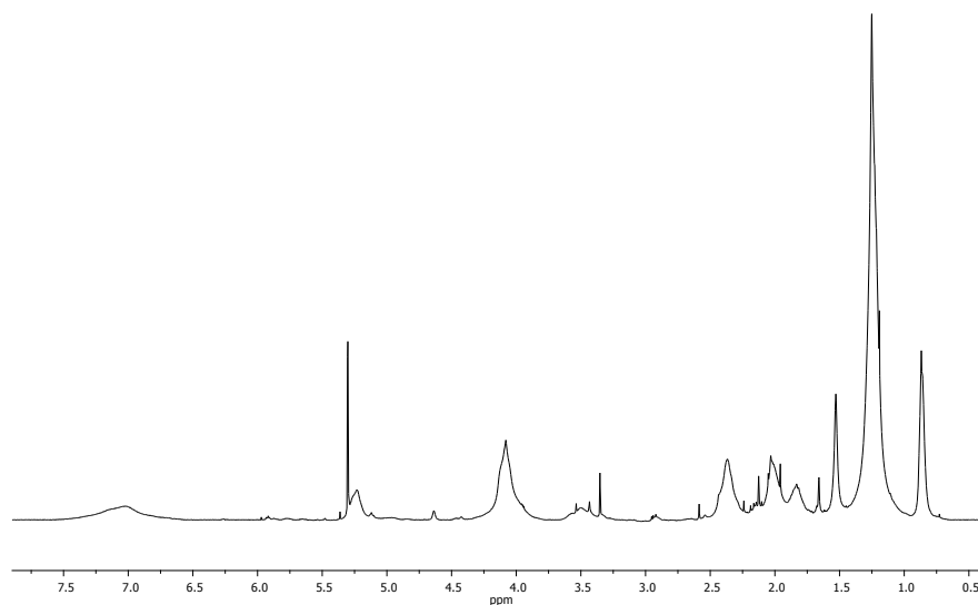
Figure S2. ^1\text{H} NMR (500 MHz, \text{CD}_2\text{Cl}_2 ): \delta 7.5-6.7 ( \text{CH}_{\text{aromatic}} ), 5.96 ( \text{CH} ), 5.17 ( \text{CH}_{\text{COD}} ), 4.0 ( \text{CH}_3 ), 3.5-3.35 ( \text{CH}_2 ), 2.41 ( \text{CH}_{2,\text{COD}} ), 2.08 ( \text{CH}_{2,\text{COD}} ), 2.42-1.00 ( \text{CH}_2 ), 0.88 ( \text{CH}_3 ).
