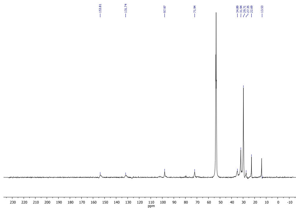
Figure S3. ^{13}\text{C} NMR (126 MHz, \text{CD}_2\text{Cl}_2 ) \delta 153.8, 131.7, 98.0, 71.9, 34.9, 31.9, 29.7, 27.4, 22.7, 13.5.
