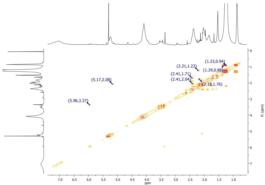
Figure S5. COSY NMR spectrum of 1 ( \text{CD}_2\text{Cl}_2 )
