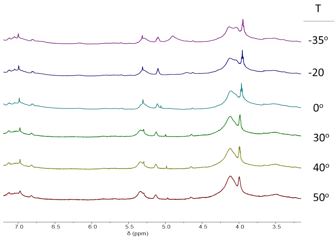
Figure S4. VT ^1\text{H} NMR spectrum of 1 ( \text{CD}_2\text{Cl}_2 )
