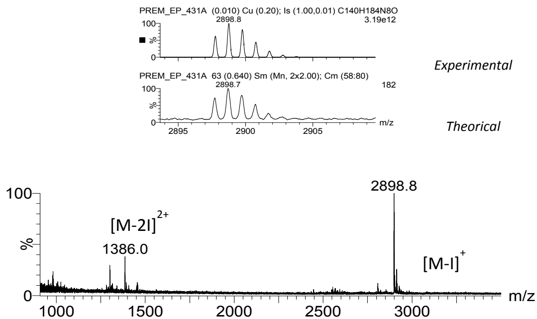
Figure S6. Time-Of-Flight Mass Spectrum (TOF-MS) of 1
