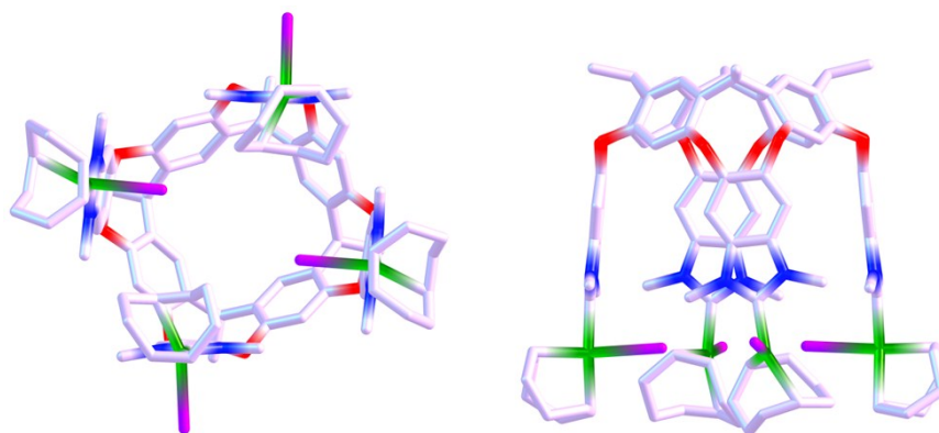
Vase_5 (4.0 kcal/mol)
