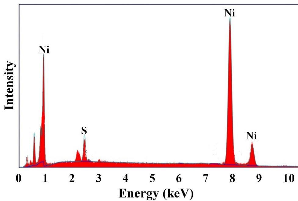
Fig. S1 EDX spectrum of \text{Ni}_3\text{S}_2 nanostructure material.
