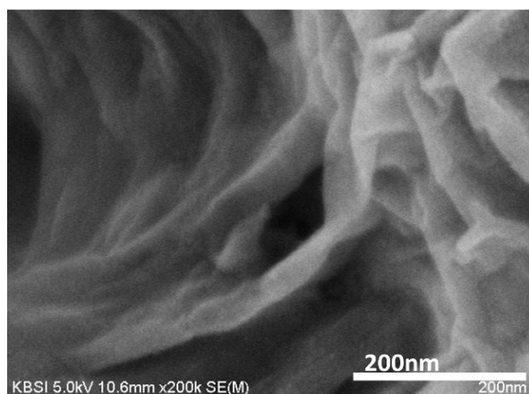
Fig. S1. FE-SEM image of NiMoO 4 nanosheet structure after 5000 cycles.
