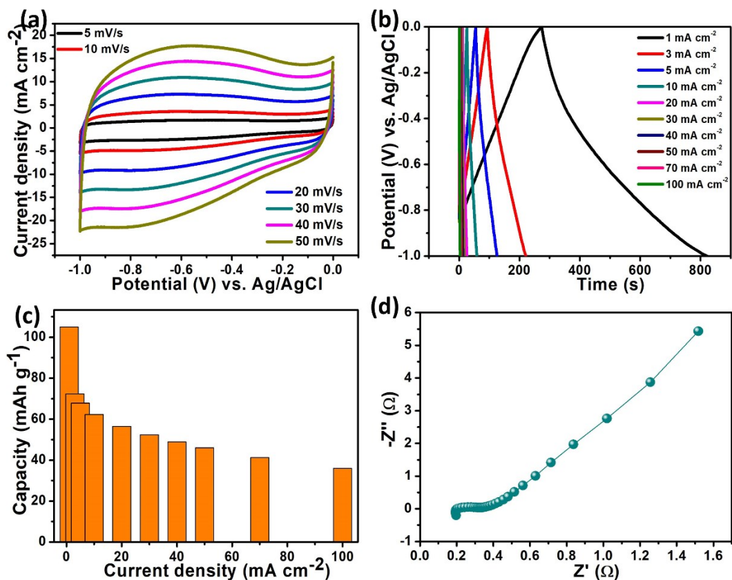
Fig. S2. (a-b) CV and GCD plots of MCG-ink in 3 M KOH electrolyte solution, (c-d) corresponding current density vs specific capacity of MCG-ink and EIS spectrum.
