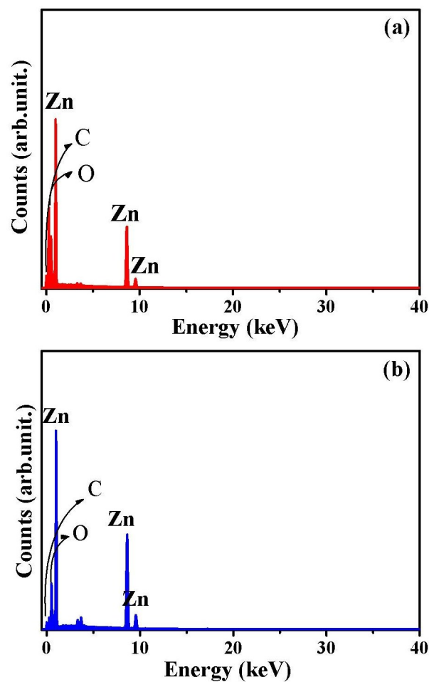
Figure S1. Semi-quantitative analyses performed by EDS demonstrating spectrum of (a) AGZ and (b) KGZ .
