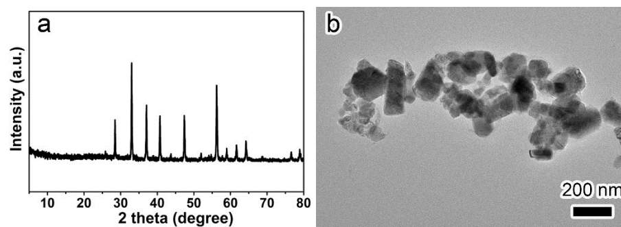
Fig. S1 The XRD pattern (a) and TEM image (b) of FeS 2 nanosheets.
