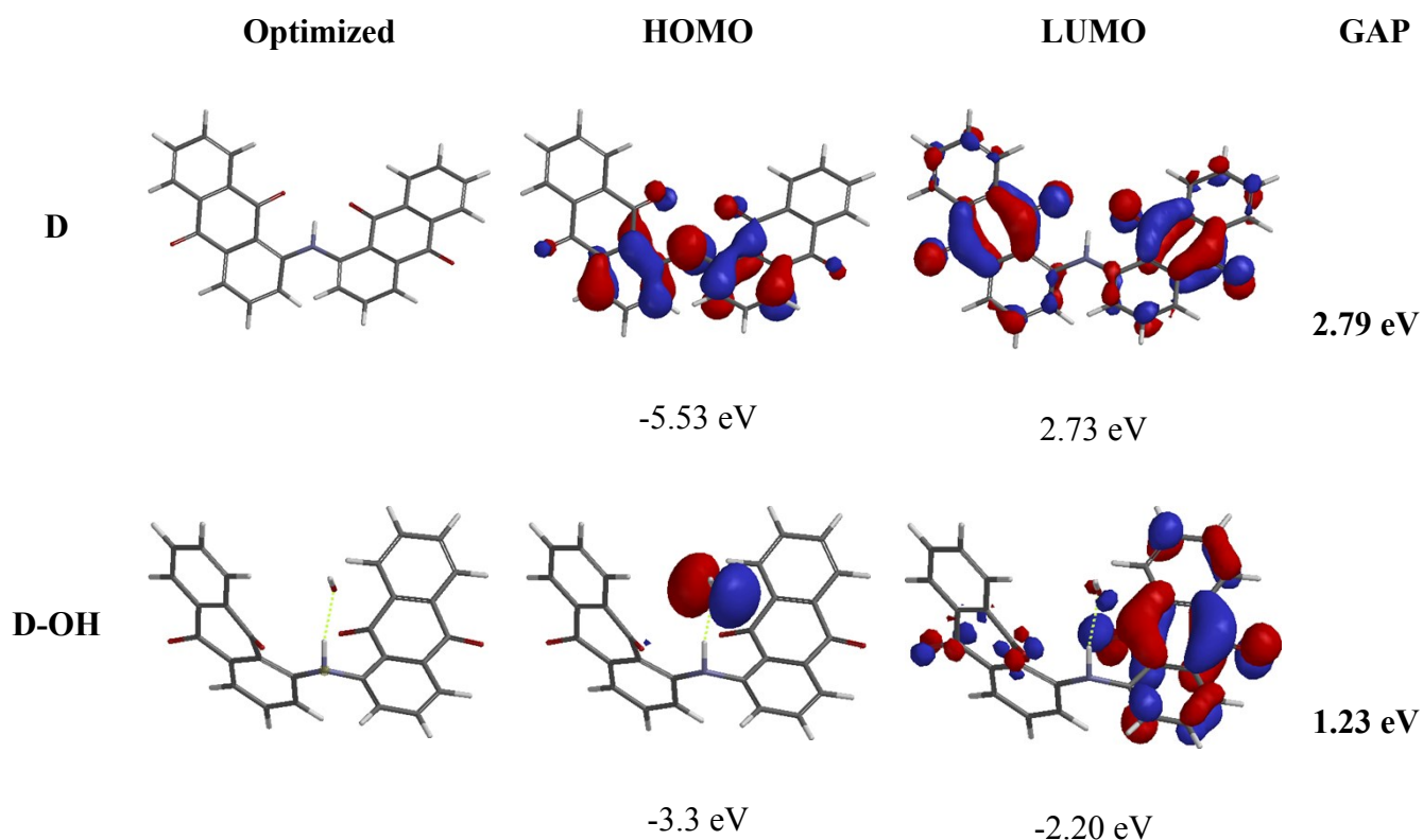
Figure S1: Excited state HOMO and LUMO diagrams of D and D-OH in DMSO
