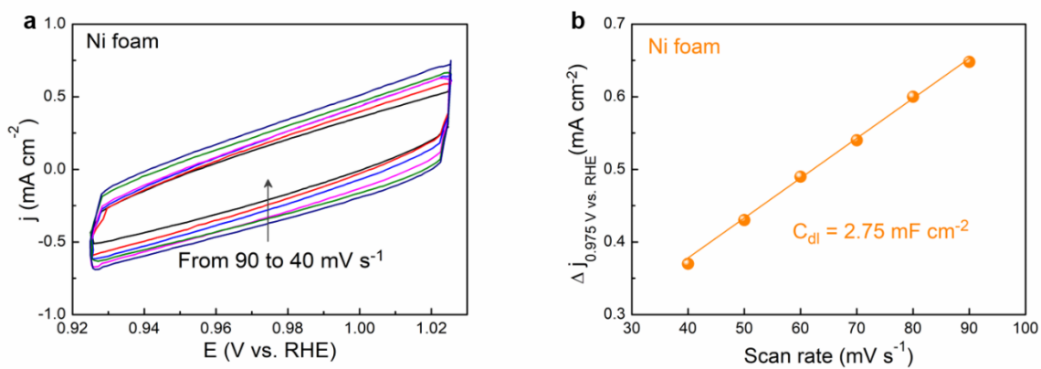
Fig. S10 (a) CV curves of Ni foam at scan rates ranging from 40 \text{mV s}^{-1} to 90 \text{mV s}^{-1} with an interval point of 10 \text{mV s}^{-1} . (b) Calculation of C_{dl} for Ni foam by plotting the capacitive current density against the scan rate to fit a linear regression.
