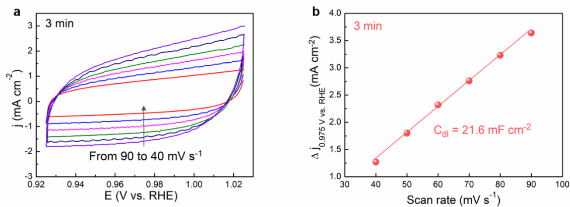
Fig. S13 (a) CV curves of S-(Ni,Fe)OOH (reaction time: 3 min) at scan rates ranging from 40 mV s -1 to 90 mV s -1 with an interval point of 10 mV s -1 . (b) Calculation of C_{dl} for the 3-minute sample by plotting the capacitive current density against the scan rate to fit a linear regression.
