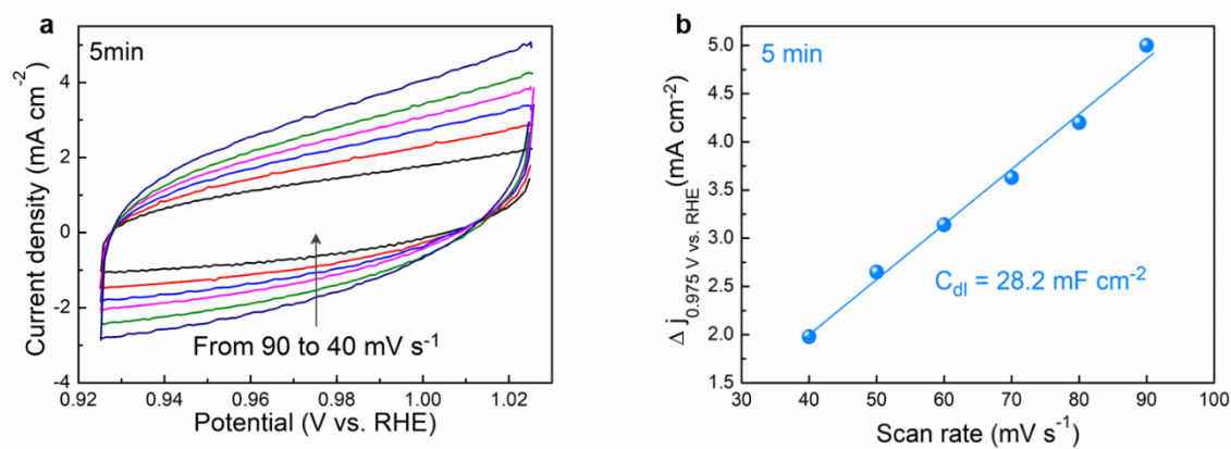
Fig. S14 (a) CV curves of S-(Ni,Fe)OOH (reaction time: 5 min) at scan rates ranging from 40 mV s -1 to 90 mV s -1 with an interval point of 10 mV s -1 . (b) Calculation of C dl for the 5-minute sample by plotting the capacitive current density against the scan rate to fit a linear regression.
