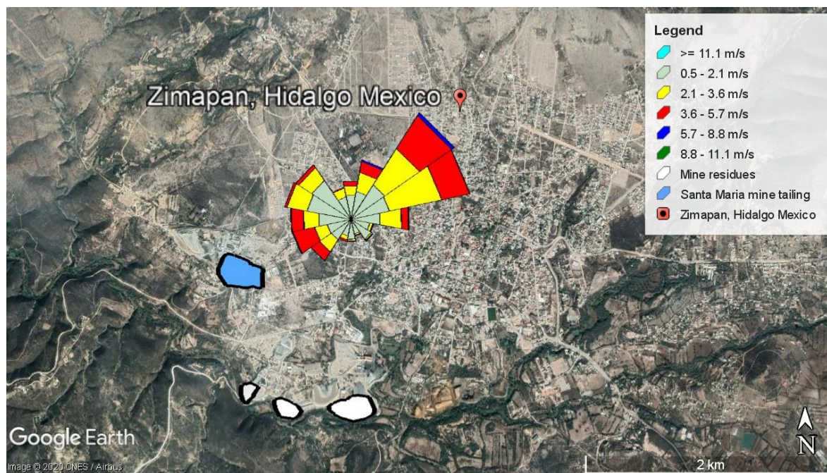
Fig. S2. Santa Maria mine residues location and the wind rose at Zimapan, Hidalgo, during the dry season.
