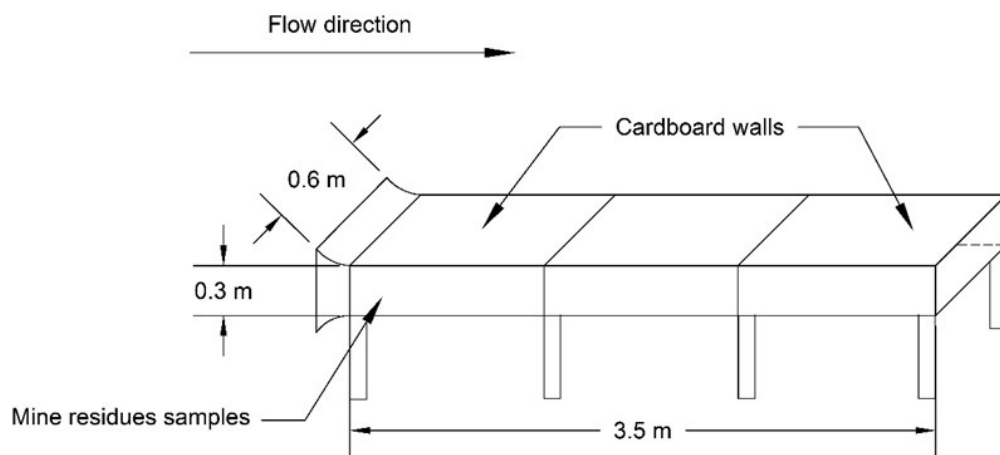
Fig. S3. Wind tunnel used for simulation of the dispersion of mine residues.
