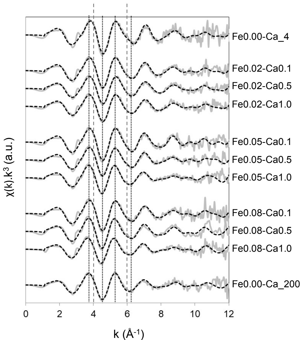
Figure SI 8 – Calcium K-edge EXAFS of Fe-OM-Ca aggregates. Grey solid lines are the experimental data and the black dotted lines are the fit results.
