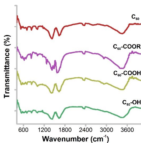
Fig. S1 IR spectra of fullerene samples.
