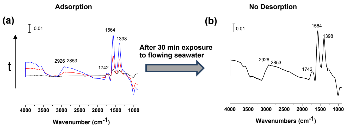
Fig. S1 ATR-FTIR spectra of FA adsorption onto PVP-coated Fe 3 O 4 NPs (a) 10 ppm FA flow for adsorption, (b) sea water flow for desorption; black, red and blue lines represent 15, 90 and 120 min, respectively.
