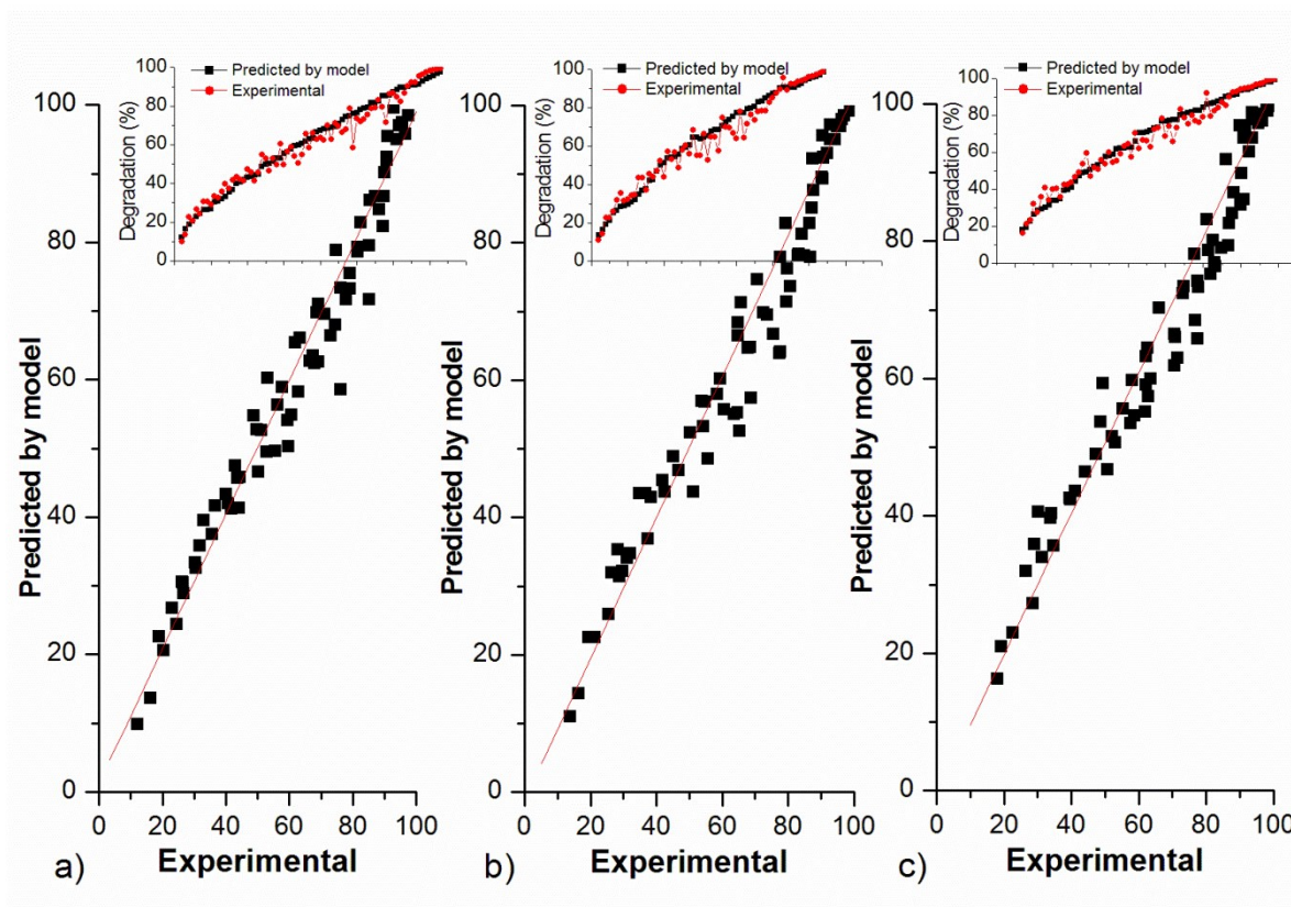
Figure S1. Correlation between the experimental and the predicted values in a regression model for: (a) UV/H 2 O 2 (b) UV/S 2 O 8 2- and (c) UV/HSO 5 - processes
