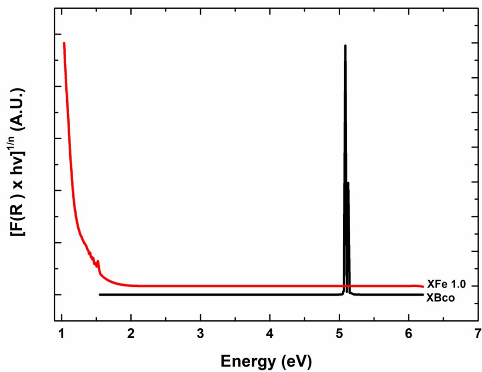
Figure S1 Band-gap diagram for the XFe 1.0 and XBco materials
