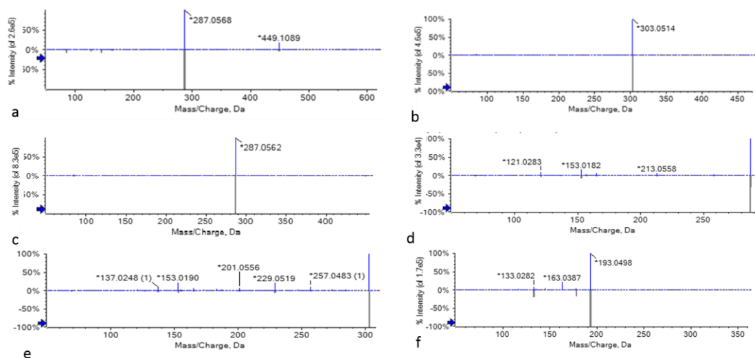
Figure S1 TOF MS analysis of flavonoids in the aqueous extract of mulberry leaves including rutin (a), isoquercetin (b), astragalin (c), kaempferol (d), quercetin (e), and scopolamine (f).
