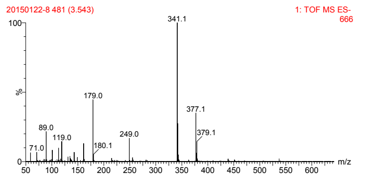
Figure S1. The mass fragmentation patterns of reuteransucrase catalyzed gluco-oligomer mixtures.
