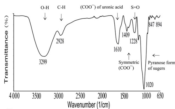
Fig. S2. FT-IR spectra of GOP-1.
