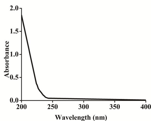
Fig. S1. Ultraviolet spectra of GOP-1 in the range of 200-400 nm
