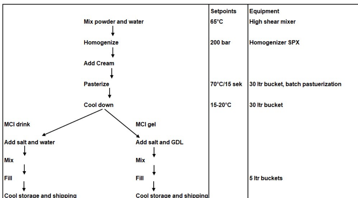
Suppl. Fig 1. Process diagram of production of MCI Drink and MCI Gel
