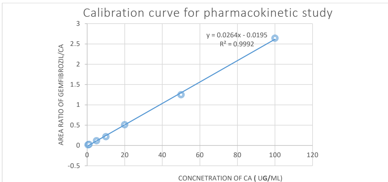
Figure. Calibration curve of the plasma CA concentration versus HPLC obtained ratio of Area of Gemfibrozil to CA
