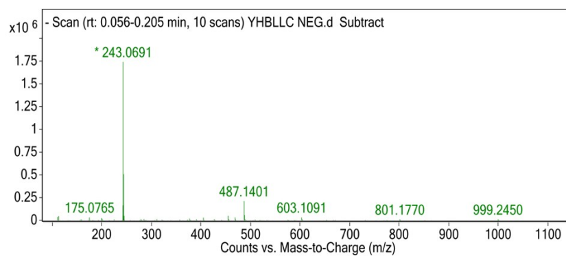
A. Negative Ion Spectrograph
