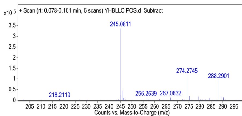
B. Positive Ion Spectrograph
