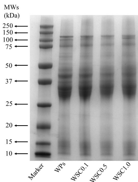
Fig. S1. SDS-PAGE profiles of WPs and silybin loaded WSCs.
