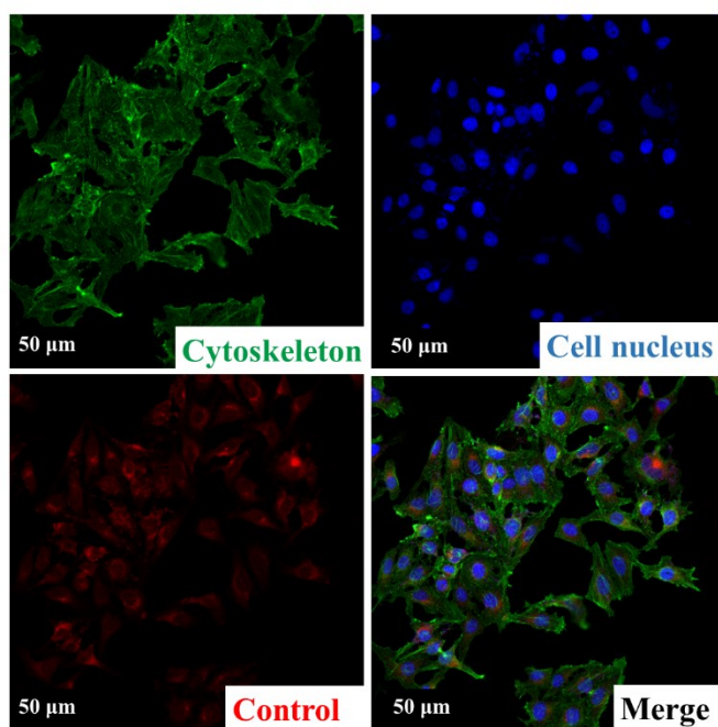
Fig. S2. CLSM images of HepG-2 cells cultured with non-silybin loaded WSC1.0.
