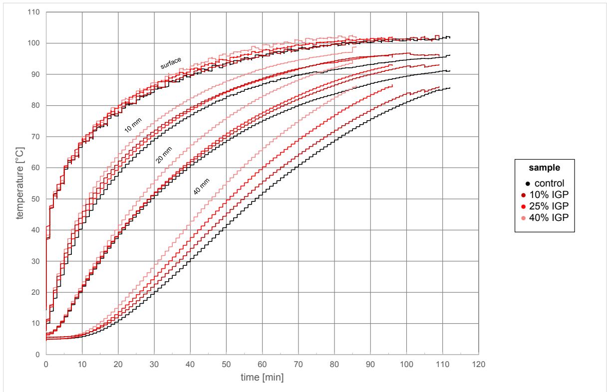
4 Figure A2: Thermal profiles of meat product samples with various content of inert material 5 IGP (labels of samples see Table 1 ) in a casing with a diameter of 90 mm.
