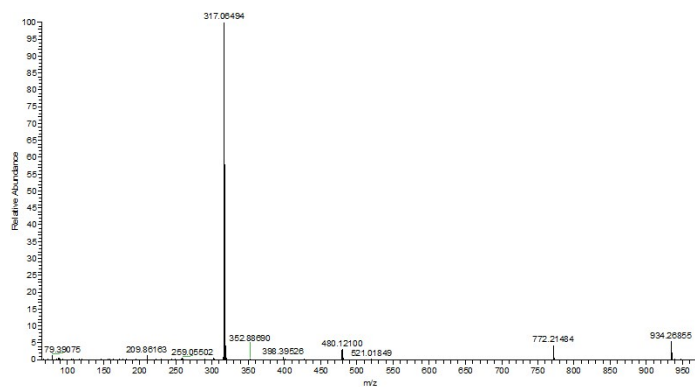
Supplementary Figure 1 The HPLC and MALDI-TOF-MS of anthocyanins from Lycium ruthenicum Murray. (A) HPLC of the crude extract of anthocyanins. (B) HPLC of the Pt3G. (C) MALDI-TOF-MS of Pt3G.
