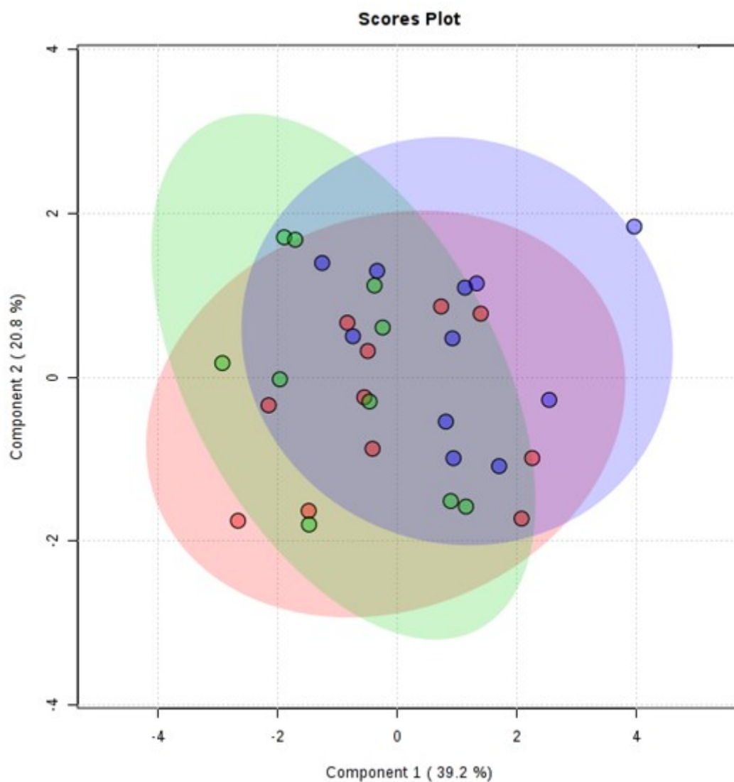
Figure 1. Comparison of Partial Least Square Discriminant Analysis (PLS-DA) in metabolites between groups
