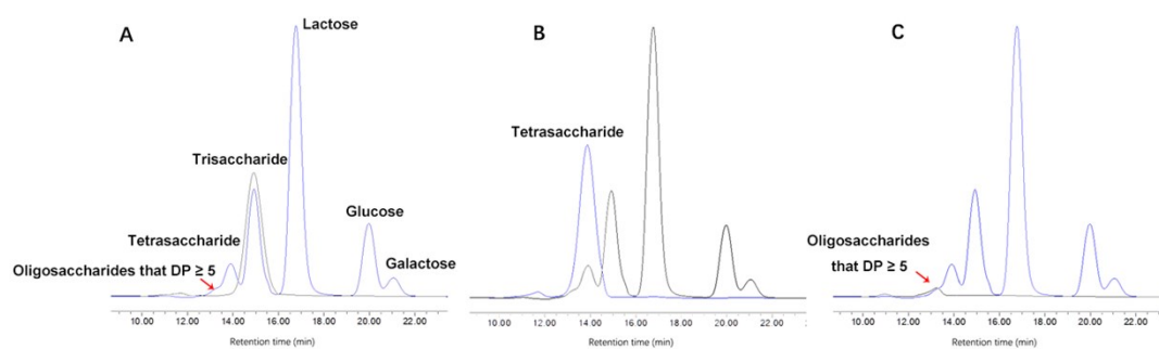
Figure S1. HPLC of single component of trisaccharide (A), tetrasaccharide (B), and oligosaccharides that DP \geq 5 (C). The lactose hydrolysate was used for an reference, i.e. the blue line in (A), (C) and black line in (B).
