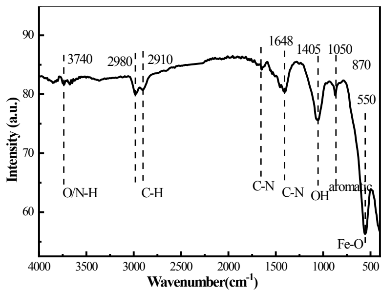
Figure S1 The FTIR result of ATFS.
