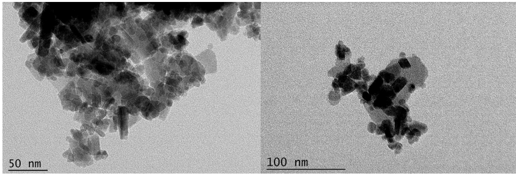
Figure S4 TEM results of ATFS.
