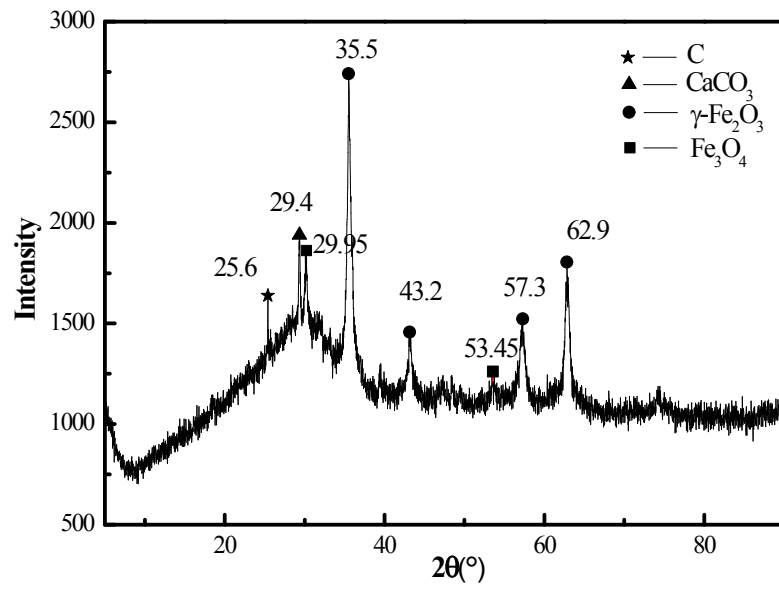
Figure S2 XRD results of ATFS.
