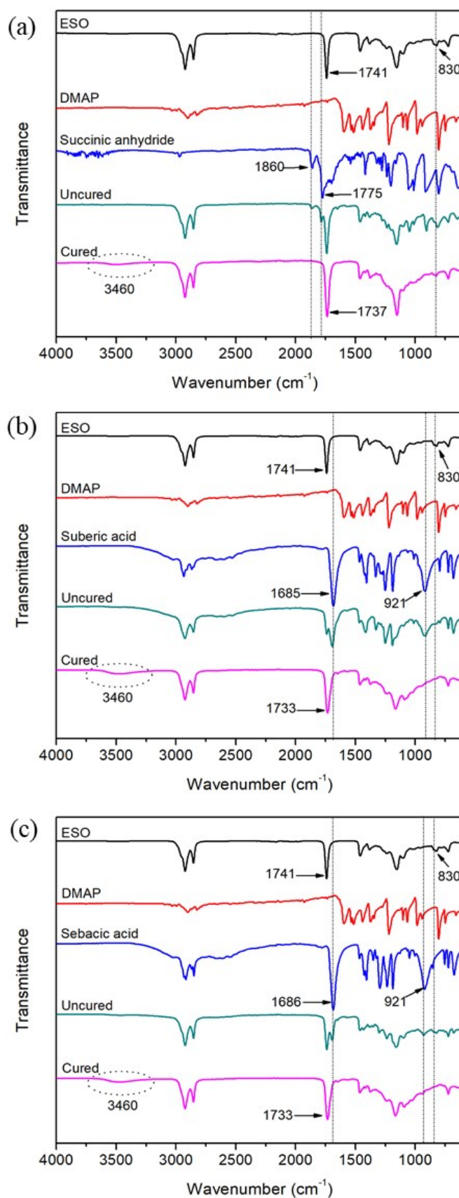
Fig. S2 FTIR spectra of ESO cured with different crosslinkers.
