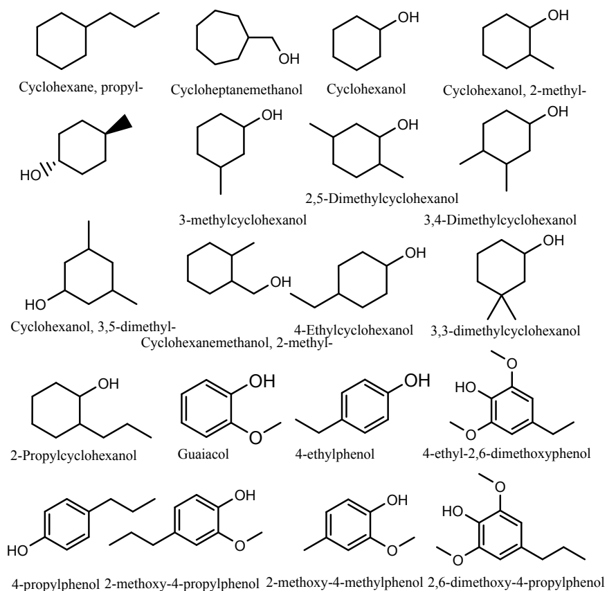
Figure.S1 the monomers structure produced by ISU PL SCM-DHDO at 4h 300°C
