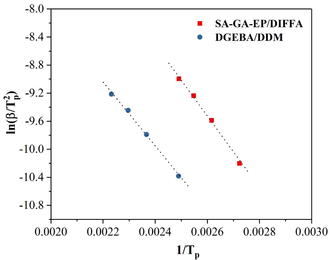
Fig. S2 Linear plots of \ln(\beta/T_p^2) as a function of 1/T_p of DGBEA/DDM and SA-GA-EP/DIFFA based on Kissinger's method.
