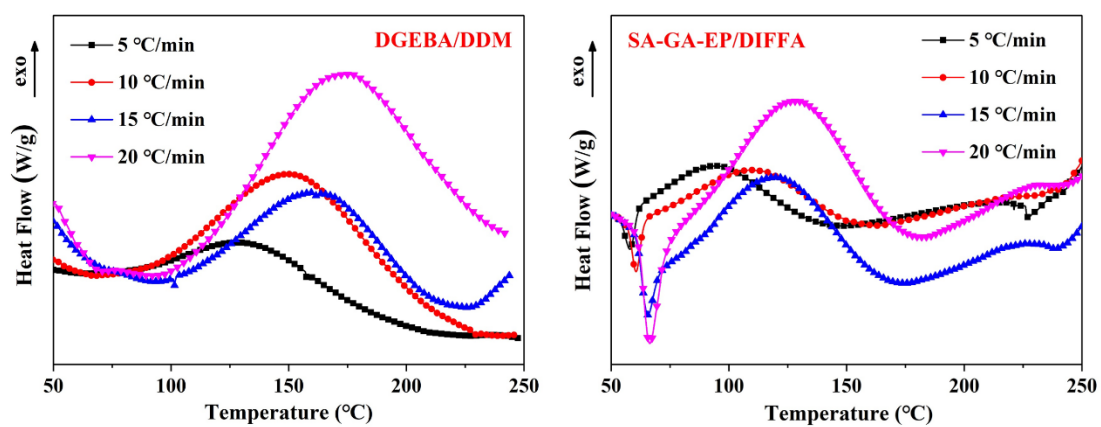
Fig. S1 DSC thermograms of DGEBA/DDM and SA-GA-EP/DIFFA at various heating rates.
