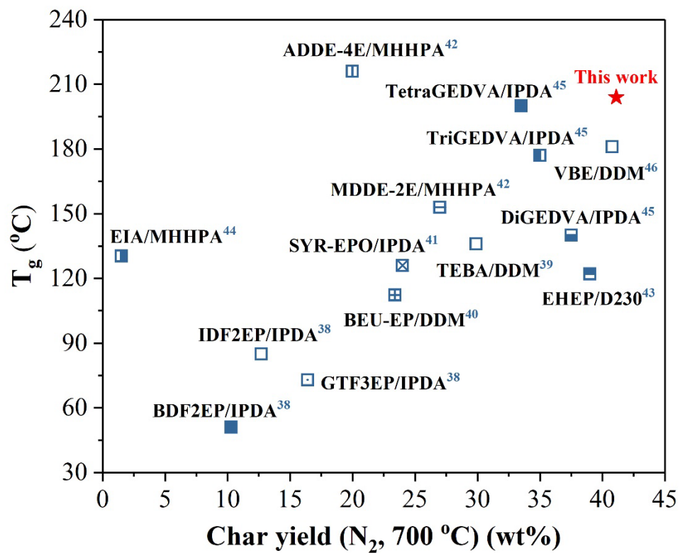
Fig. S3 Comparison of T_g and char yield between SA-GA-EP/DIFFA and previously reported results.
