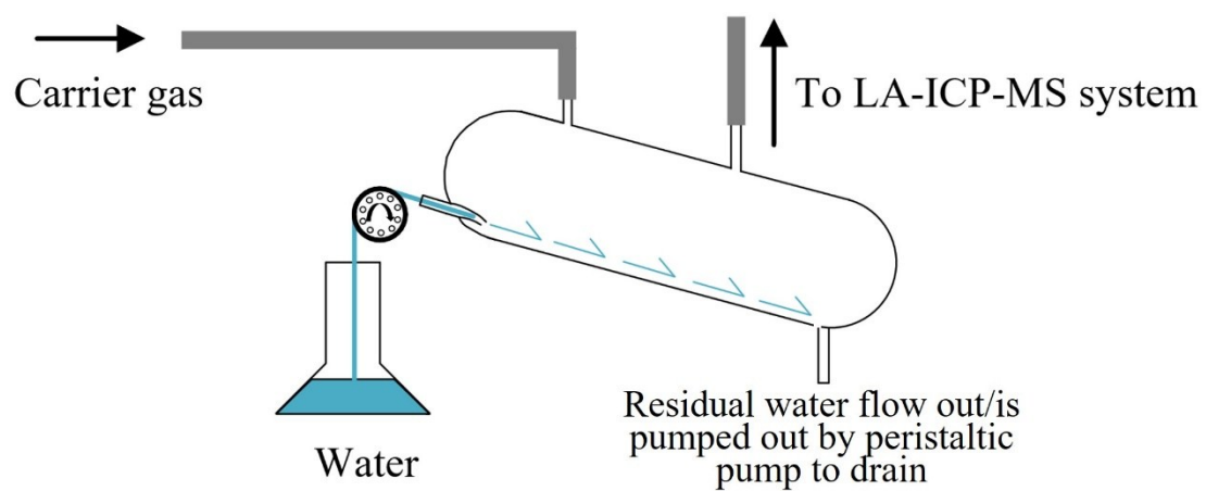
Figure S1. Schematic of the in-house water vapor introduction system. 1
