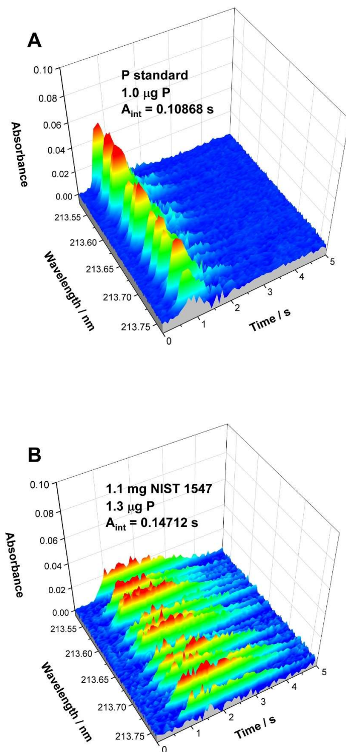
Figure S1. Wavelength- and time-resolved spectra recorded for (A) 1.0 \mu\text{g} of P introduced as standard solution with 10 \mu\text{g Au} / 15 \mu\text{g Ca} ; and (B) 1.1 mg of CRM NIST 1547 with 10 \mu\text{g Au} under the temperature conditions described in Table 1.
