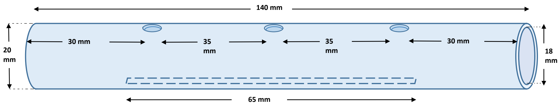
Slotted Quartz Tube used in the system
