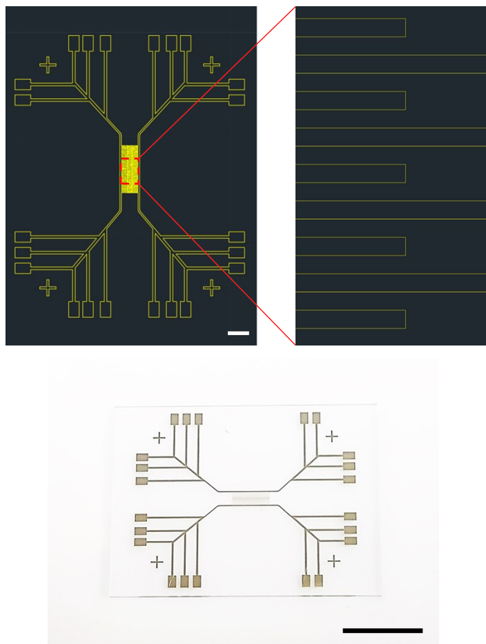
Fig. S1. Cr/Au patterned glass slide. Scale bars are 2mm (top) and 1cm (bottom).
