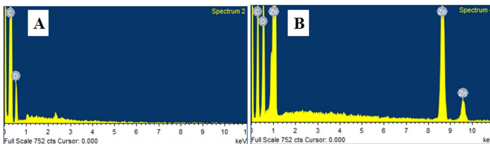
Fig. S4 EDS spectra of (A) rGO and (B) ZSs@1rGO.
