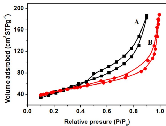
Fig. S2 N 2 adsorption isotherm of (A) GO and (B) rGO.
