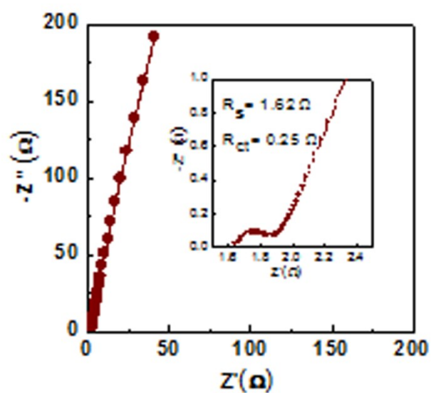
Fig. S3. Nyquist plot of rGO modified GCE.
