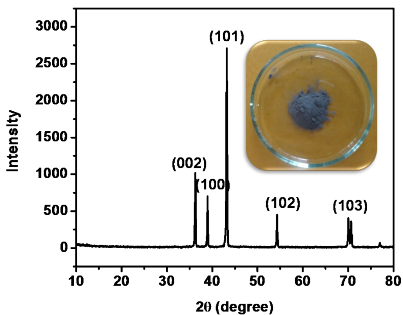
Fig. S1 XRD pattern of Zn dust. Inset is the photographic image of Zn dust.
