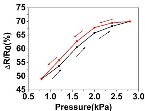
Figure S2: Hysteresis curve of normalised resistance against applied external pressure.
