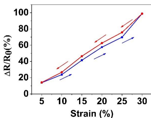
Figure S1: Hysteresis curve of normalised resistance against tensile strain (%).
