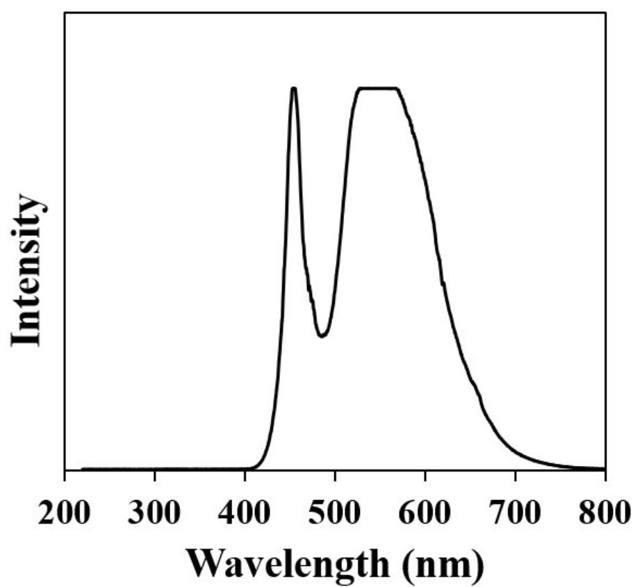
Fig. S1: Spectrum of LED used in photocatalytic system
