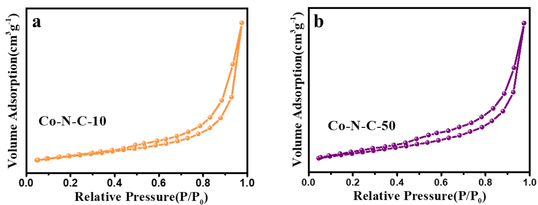
Fig. S2. Nitrogen adsorption–desorption isotherms of Co-N-C-10 and Co-N-C-50.
