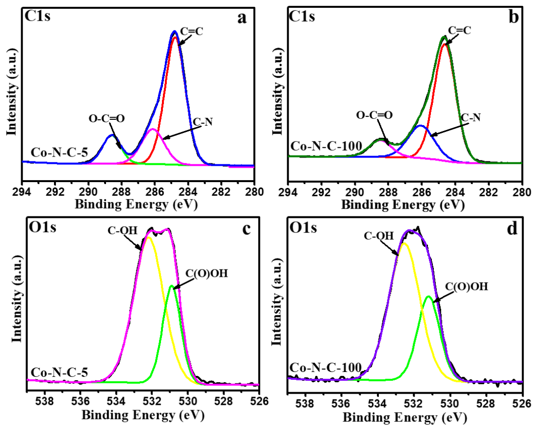
Fig. S3. XPS spectra of as-prepared catalysts. (a) C 1s XPS spectrum and (c) O 1s XPS spectrum of the sample Co-N-C-5; (b) C 1s XPS spectrum and (d) O 1s XPS spectrum of the sample Co-N-C-100.
