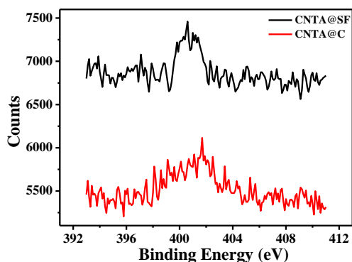
Figure S2. N 1s spectra of CNTA@SF and CNTA@C composites.
