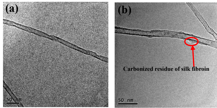
Figure S3. TEM images of CNTA@SF and CNTA@C composites
